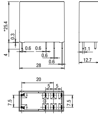
RF2V (PC board terminal) Standard (without LED/diode)
