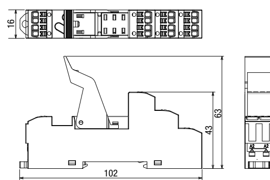
Marking Plate (integrated with release lever)
