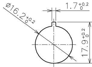
Panel cut-out (Applicable to IEC60947-5-1)
